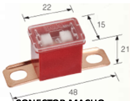
CONECTOR MACHO 48 MM
